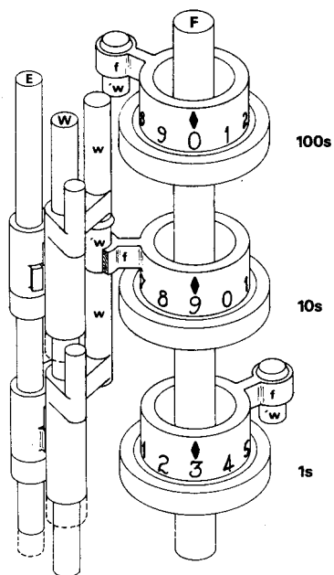
Fig. 7. Anticipating carry. The movable wire 'w carried in the arm of the figure wheel can interpose between the fixed wires w to propagate a carry through several cages. In the figure, a carry is generated in the units cage. Because the 10s figure wheel stands at nine, a carry is propagated to the 100s cage. The 100s figure wheel does not stand at nine and therefore breaks the chain of carry propagation.
