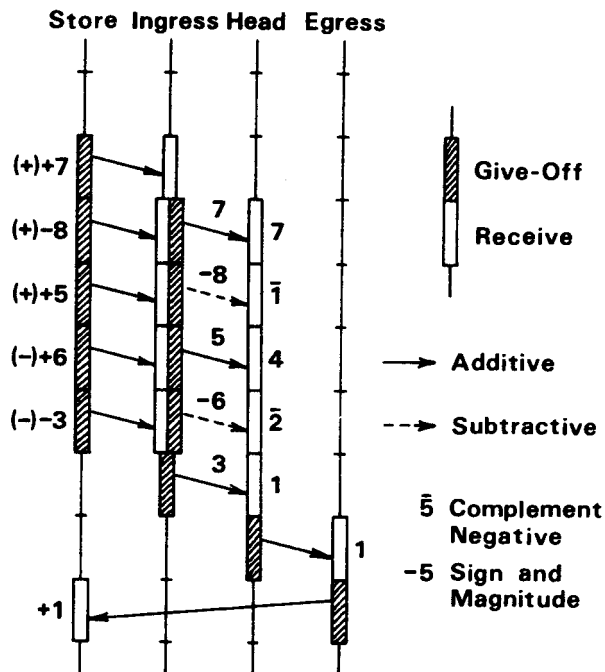
Fig. 14. Overlapping of functions in the pipeline for signed addition. Five operands are accumulated, and only the result is returned to the store.
