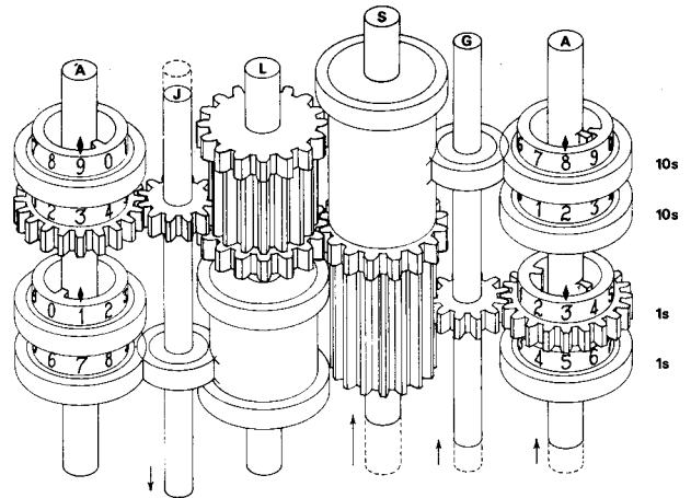
Fig. 4. The process of stepping, or multiplication, and division by 10. The long pinions S are raised with their axis to engage the long pinions L in the cage above. A number given off will therefore be stepped up a cage, or multiplied by 10. A transfer in the reverse direction will divide by 10.
