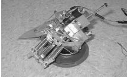
Figure 7: Photo of 2 nd Generation hopper in compressed state. The outer shell is removed for clarity.
