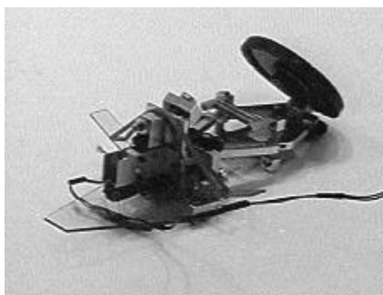
Figure 17: Posture at end of self-righting phase I.
